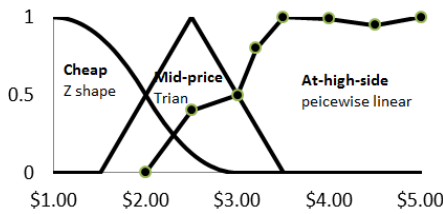
Figure 2. Examples of membership functions for the linguistic variable: oil_price
